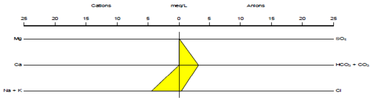
Figure 15. Stiff diagram for Power Mountain sampling location PM-11 (WVDEP, 2009)
