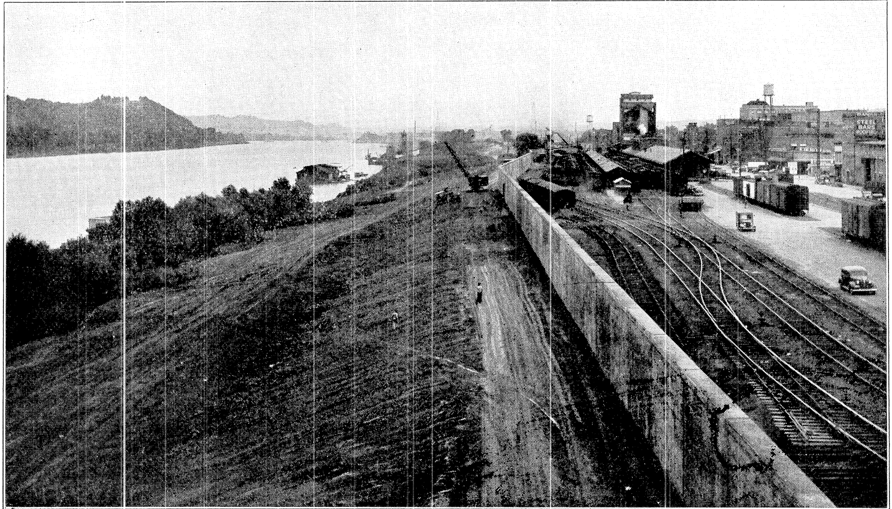
View Looking North from Sixth Street Bridge in Huntington, Showing Part of Completed Flood Wall.
